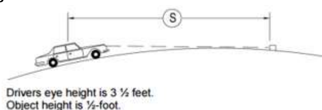
Crest Curve Stopping Sight Distance
